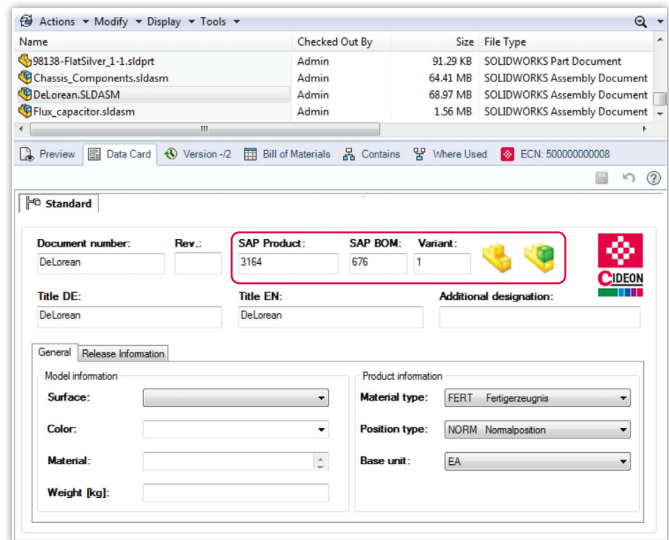
Additional SAP information in the data card of an assembly
