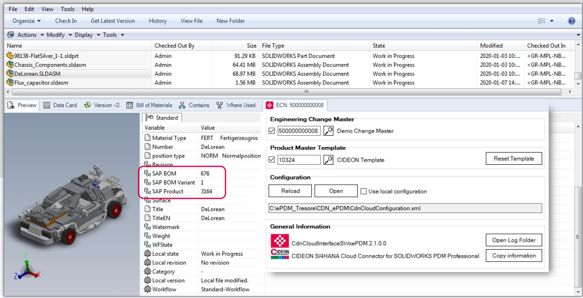
Additional SAP information in the variables of an SOLIDWORKS assembly and the connector tab with controls and SAP information
